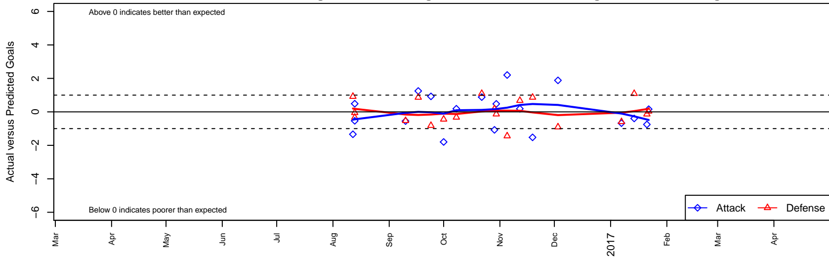
IFC Select Red G03 Dots are actual minus expected GF (blue circles) and GA (red triangles). Blue line is smoothed change in attack strength. Red is smoothed change in defense strength.
